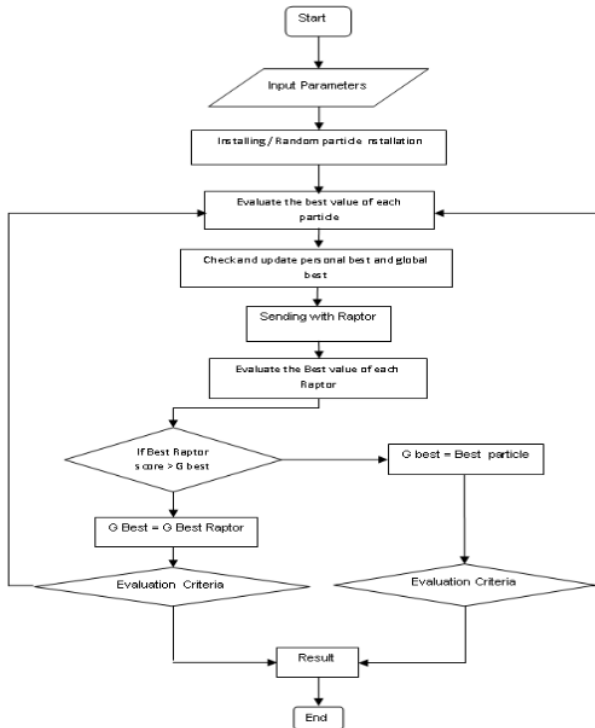
Fig. 6. Flowchart of the BSG-Starcraft PSO method
