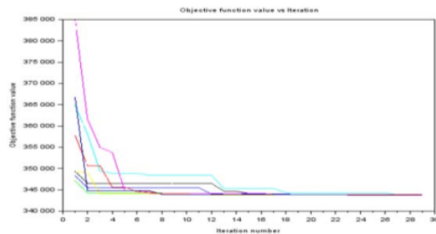
Fig.11. Convergence process with BSG Starcraft Radius PSO
